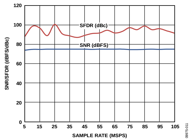
Figure 32. SNR/SFDR vs. Sample Rate with AIN = 70.1 MHz
