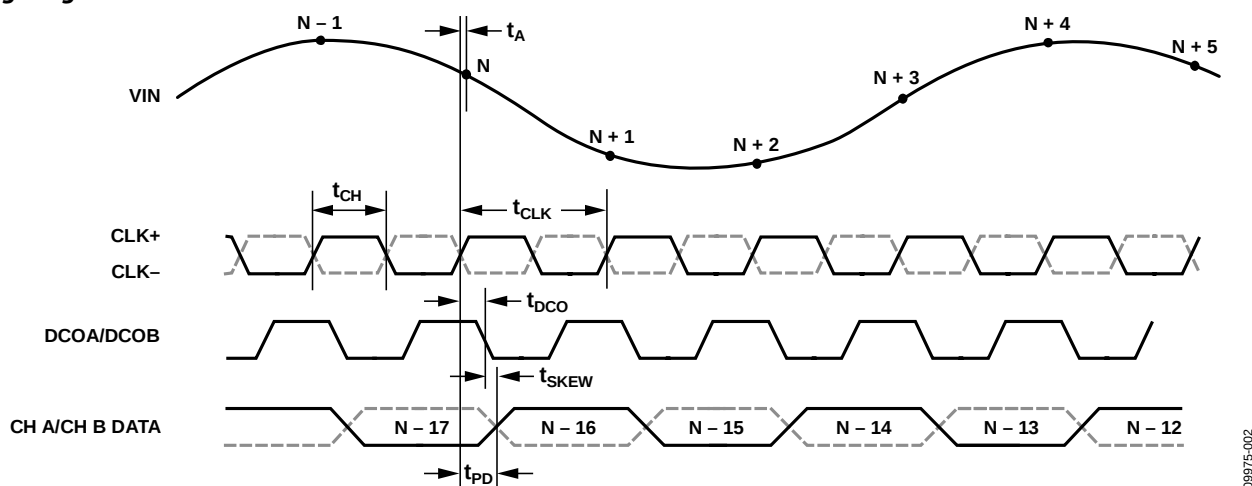
Figure 2. CMOS Default Output Mode Data Output Timing
