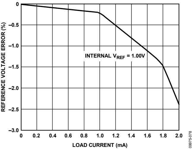
Figure 49. VREF Accuracy vs. Load Current
