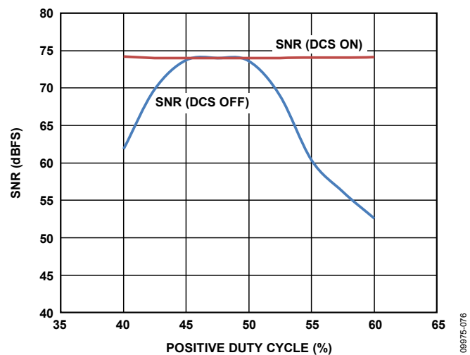
Figure 57. SNR vs. DCS On/Off
