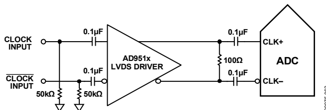
Figure 55. Differential LVDS Sample Clock (Up to 1 GHz)
