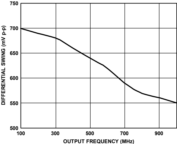
Figure 22. LVDS Differential Output Swing vs. Frequency
