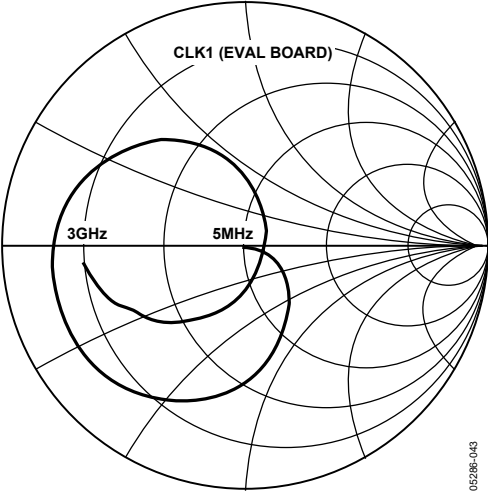
Figure 8. CLK1 Smith Chart (Evaluation Board)
