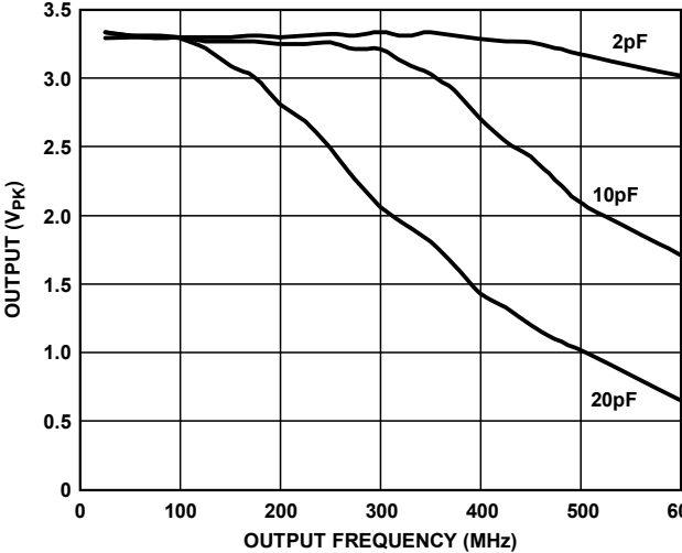
Figure 23. CMOS Single-Ended Output Swing vs. Frequency and Load
