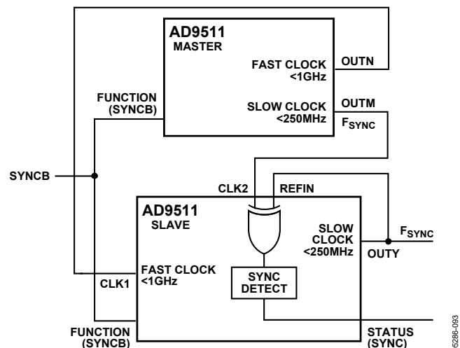
Figure 43. Multichip Synchronization
