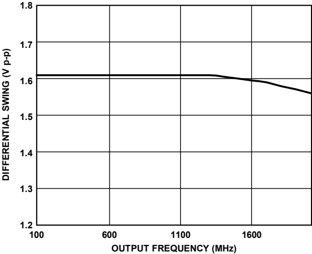
Figure 21. LVPECL Differential Output Swing vs. Frequency
