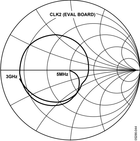
Figure 9. CLK2 Smith Chart (Evaluation Board)
