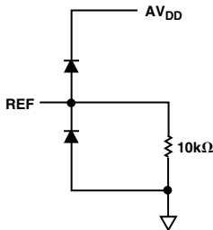
Figure 6. REF Configured as an Input
