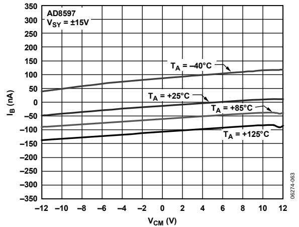
Figure 15. Input Bias Current vs. Common-Mode Voltage ( V_{CM} ) Over Temperature
