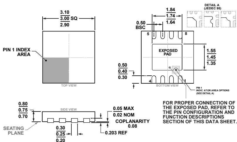
Figure 61. 8-Lead Lead Frame Chip Scale Package [LFCSFP] 3 mm × 3 mm Body and 0.75 mm Package Height (CP-8-13)
