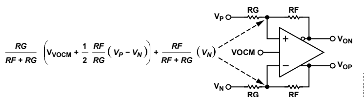
Figure 51. Voltages at the Internal Op Amp Inputs of the AD8475
