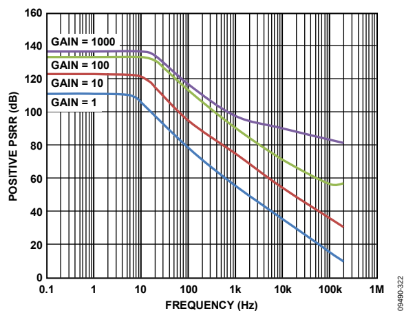
Figure 22. Positive PSRR vs. Frequency, RTI
