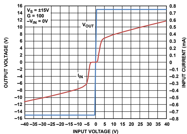
Figure 20. Input Overvoltage Performance, Dual Supply, V_S = \pm 15\text{ V} , G = 100
