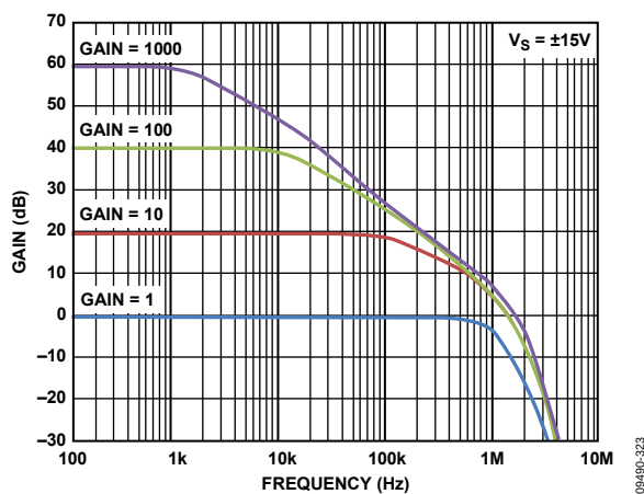
Figure 23. Gain vs. Frequency, Dual Supply, V_S = \pm 15\text{ V}
