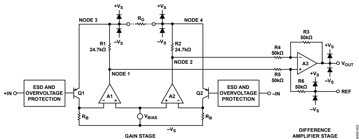
Figure 61. Simplified Schematic
