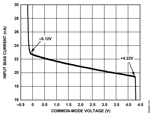
Figure 21. Input Bias Current vs. Common-Mode Voltage, Single Supply, V_S = 5\text{ V}
