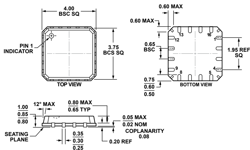
COMPLIANT TO JEDEC STANDARDS MO-263-VBBC Figure 73. 16-Lead Lead Frame Chip Scale Package [LFCSP_VQ] 4 mm × 4 mm Body, Very Thin Quad, with Hidden Paddle (CP-16-19) Dimensions shown in millimeters
