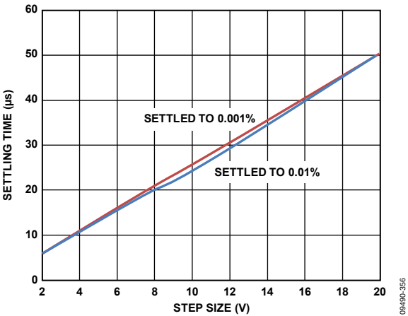
Figure 56. Settling Time vs. Step Size, Dual Supply, V_S = \pm 15\text{ V}
