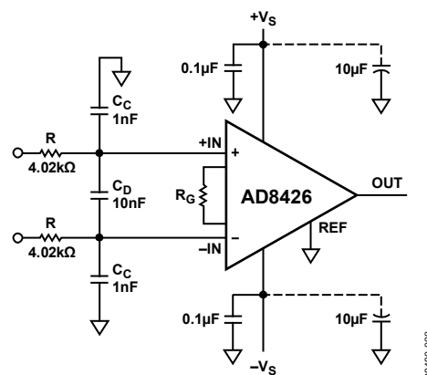
Figure 67. RFI Suppression
