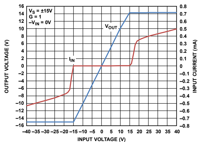
Figure 17. Input Overvoltage Performance, Dual Supply, V_S = \pm 15\text{ V} , G = 1
