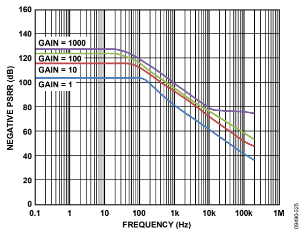
Figure 25. Negative PSRR vs. Frequency
