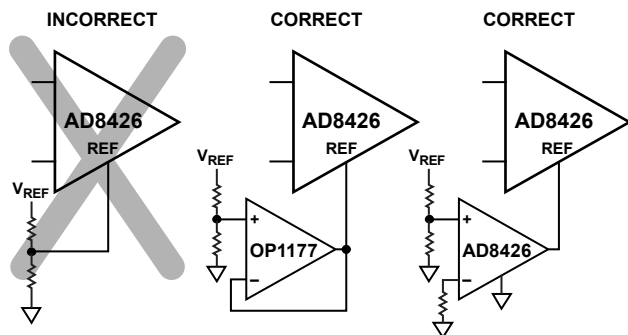
Figure 62. Driving the Reference Pin
