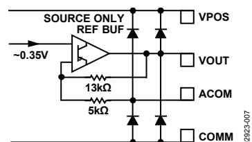
Figure 7. Circuit E
