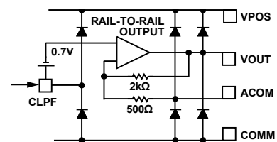
Figure 6. Circuit D
