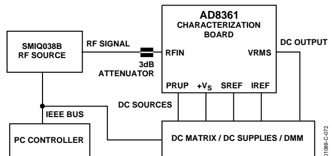
Figure 67. Characterization Setup
