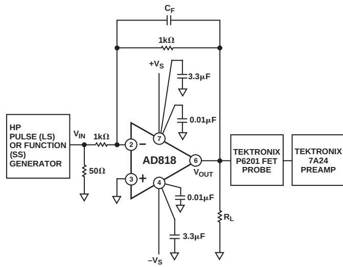
TPC 22. Inverting Amplifier Connection
