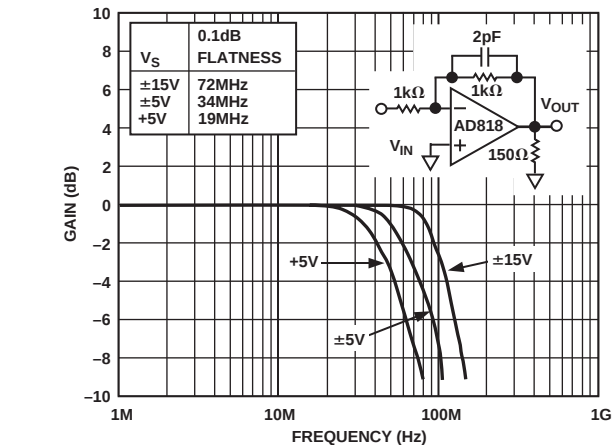
TPC 21. Closed-Loop Gain vs. Frequency ( G = -1 )
