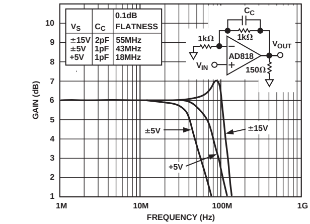
TPC 20. Closed-Loop Gain vs. Frequency ( G = +2 )
