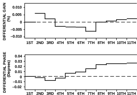
Figure 23. Differential Gain and Phase Error, G = 2 , NTSC Input Signal, R_L = 150\Omega , V_S = 5V
