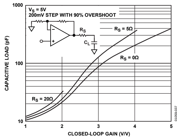
Figure 36. Capacitive Load Drive vs. Closed-Loop Gain
