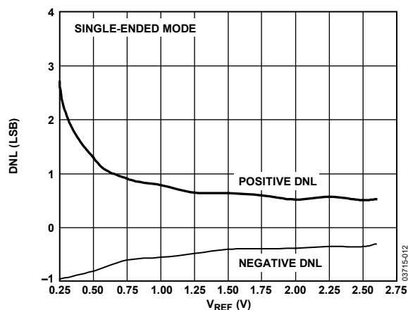
Figure 10. AD7938 DNL vs. V_{REF} for V_{DD} = 3 V
