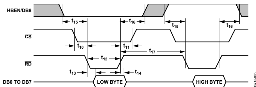
Figure 37. AD7938/AD7939 Parallel Interface—Read Cycle Timing for Byte Mode Operation ( \overline{W/\overline{B}} = 0 )
