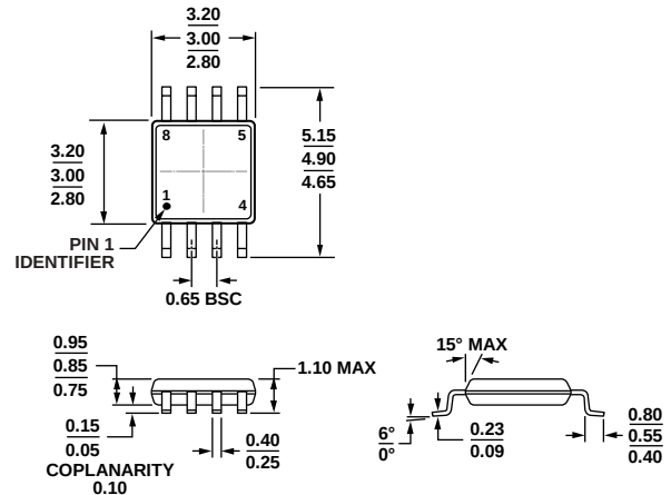
Figure 29. 8-Lead Mini Small Outline Package [MSOP] (RM-8)
