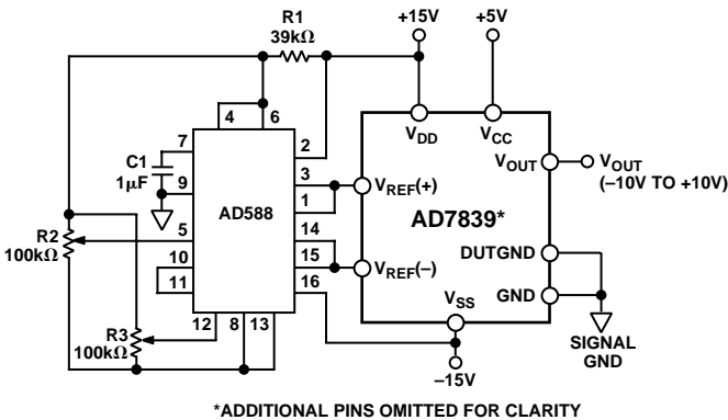
Figure 12. Bipolar \pm 10 \text{ V} Operation
