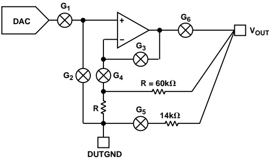
Figure 13. Block Diagram of AD7839 Output Stage
