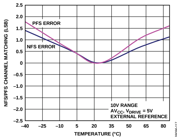
Figure 17. PFS and NFS Error Matching vs. Temperature
