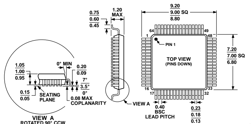
COMPLIANT TO JEDEC STANDARDS MS-026-ABD Figure 58. 64-Lead Thin Plastic Quad Flat Package [TQFP] (SU-64-1) Dimensions shown in millimeters
