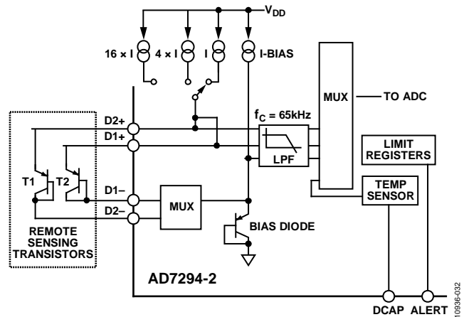
Figure 42. Internal and Remote Temperature Sensors
