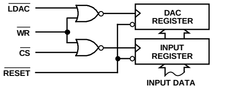
Figure 3. Input Control Logic
