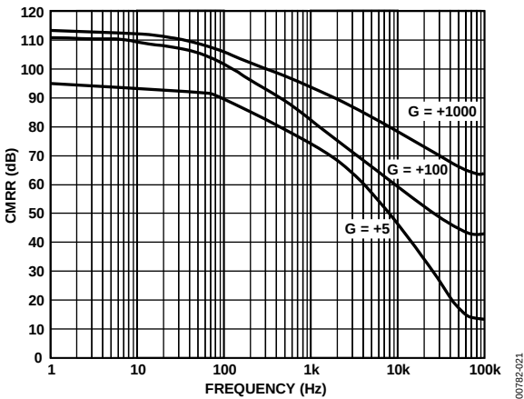
Figure 23. CMRR vs. Frequency, \pm 5 V_S ( CMV = 200\text{ mV p-p} )
