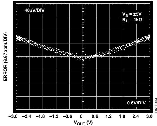
Figure 15. Gain Nonlinearity; V_S = \pm 5V , R_L = 1k\Omega
