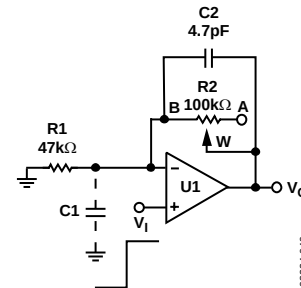
Figure 46. Typical Noninverting Gain Amplifier
