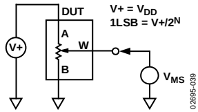
Figure 38. Potentiometer Divider Nonlinearity Error (INL, DNL)
