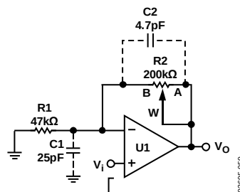
Figure 59. Typical Noninvertng Gain Amplifier
