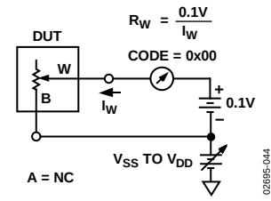
Figure 43. Incremental On Resistance
