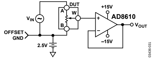
Figure 32. Test Circuit for Gain vs. Frequency
