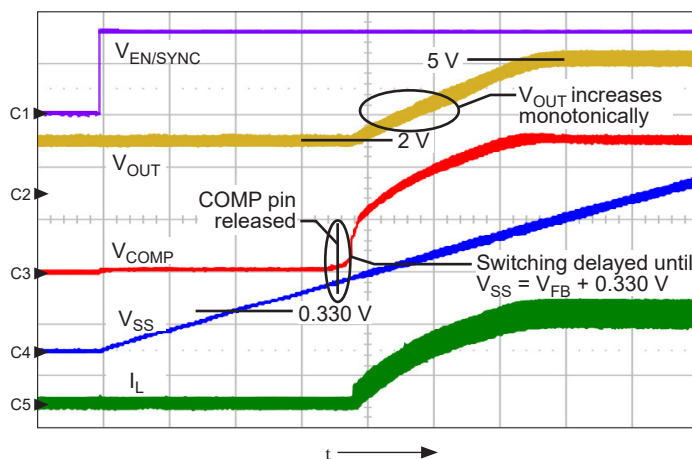
Figure 7. Startup to V_{\text{OUT}} = 5 V, with V_{\text{OUT}} pre-biased to 2 V; shows V_{\text{EN/SYNC}} (ch1, 2 V/div.), V_{\text{OUT}} (ch2, 2 V/div.), V_{\text{COMP}} (ch3, 500 mV/div.), V_{\text{SS}} (ch4, 500 mV/div.), I_{\text{L}} (ch5, 2 A/div.), t = 200 \mu s/div.
