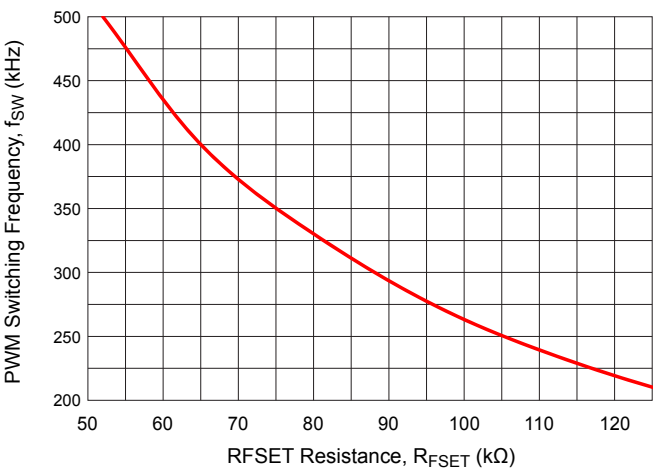
Figure 11. PWM switching frequency versus RFSET
