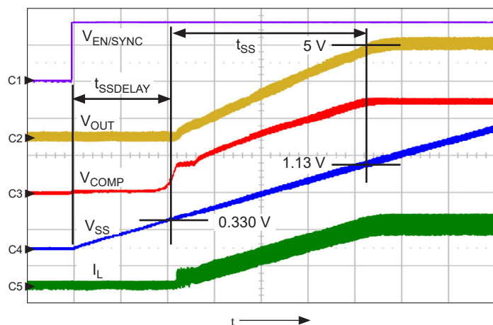
Figure 6. Startup to V_{\text{OUT}} = 5 V, 2.0 A, with C_{\text{SS}} = 22 nF; shows V_{\text{EN/SYNC}} (ch1, 2 V/div.), V_{\text{OUT}} (ch2, 2 V/div.), V_{\text{COMP}} (ch3, 500 mV/div.), V_{\text{SS}} (ch4, 500 mV/div.), I_{\text{L}} (ch5, 2 A/div.), t = 200 \mu s/div.
