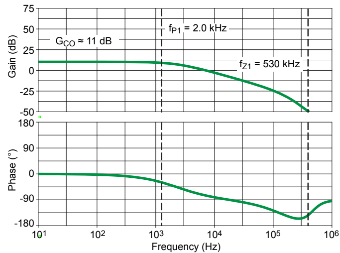
Figure 15. Control-to-output Bode plot for circuit in figure 1
