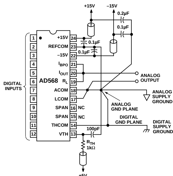
Figure 5. Bipolar Output Unbuffered \pm 1.024\text{ V}
