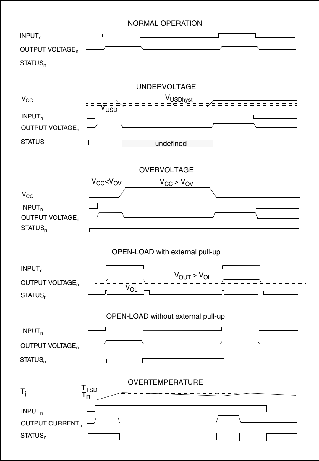
Figure 5. Waveforms
