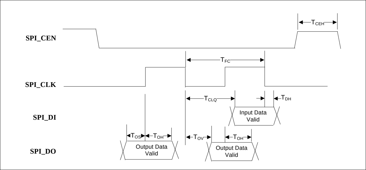
FIGURE 7-3: SPI TIMING
