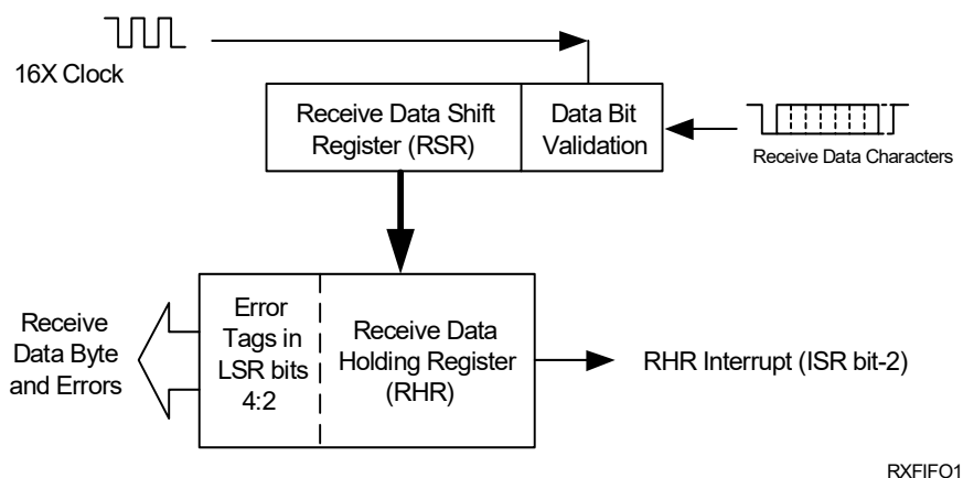
Figure 11: Receiver Operation in Non-FIFO Mode
