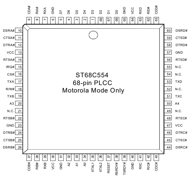
Figure 5: PLCC68 Pinout, Motorola Mode Only
