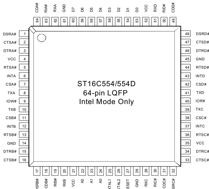
Figure 4: LQFP64 Pinout, Intel Mode Only
