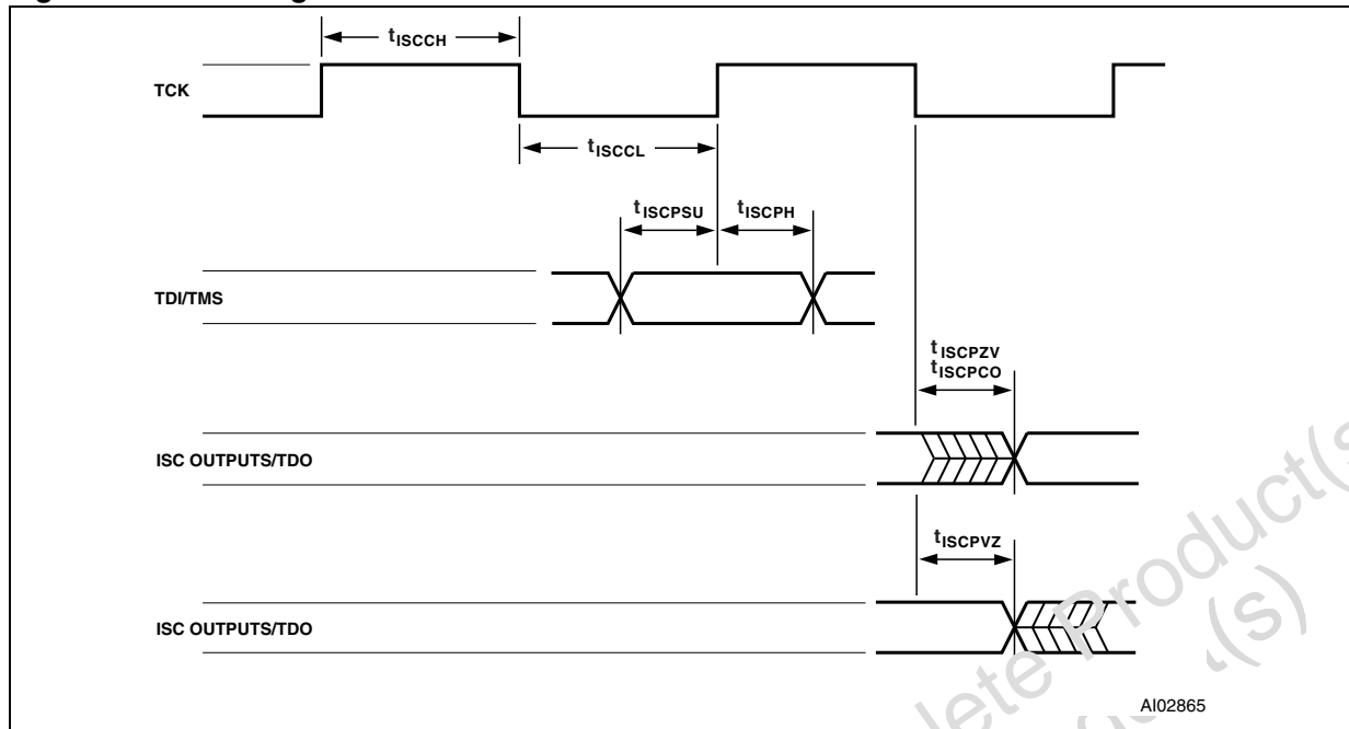
Figure 52. ISC Timing
