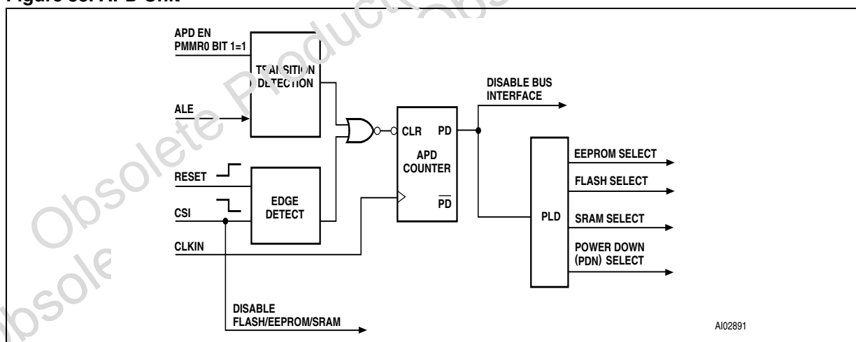
Figure 33. APD Unit
