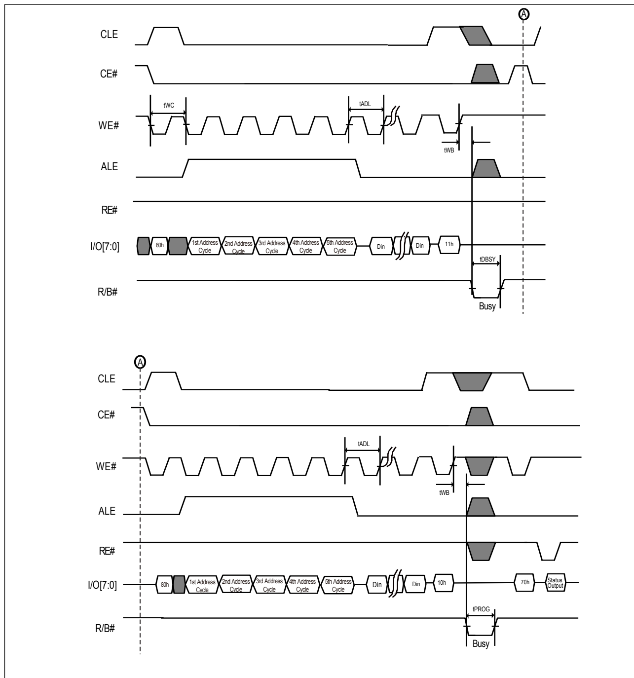
Figure 37-1. AC Waveforms for Two-plane Program (ONFI)
