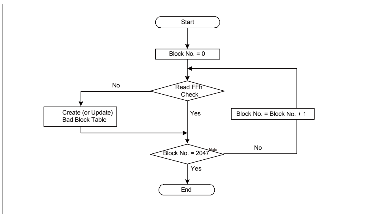
Figure 49. Bad Block Test Flow
