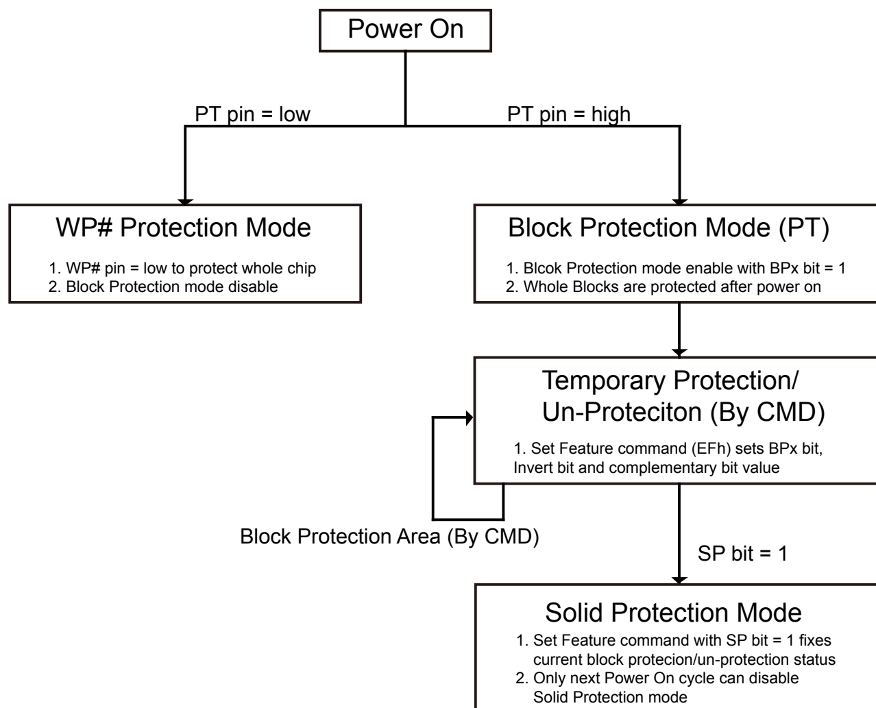
Figure 35. PT Pin and Block Protection Mode Operation
