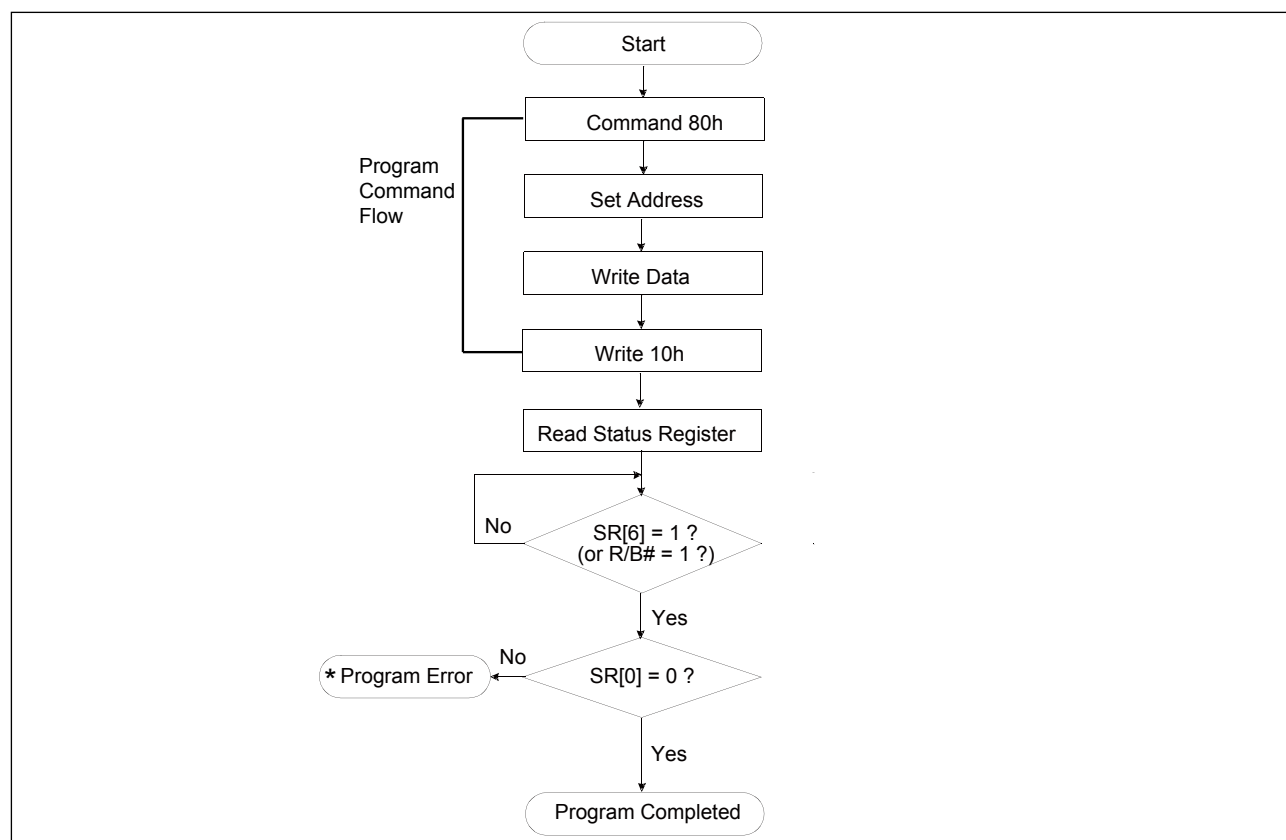
Figure 51. Program Flow Chart
