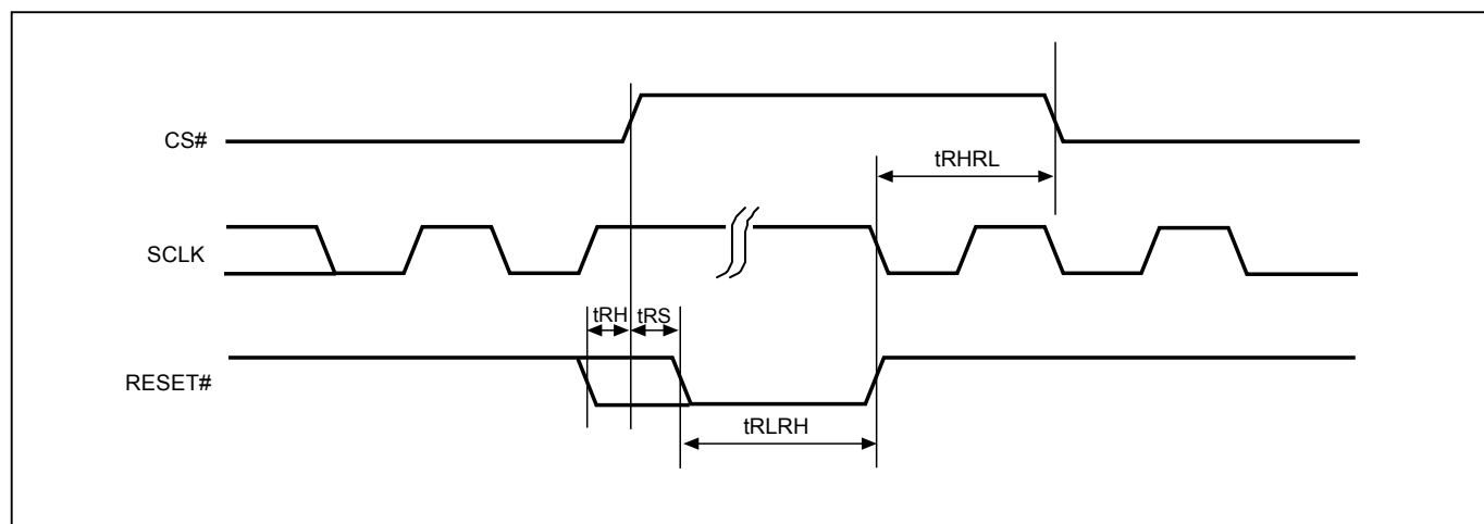
Figure 64. RESET Timing
