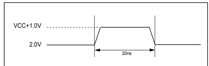
Figure 66. Maximum Positive Overshoot Waveform
