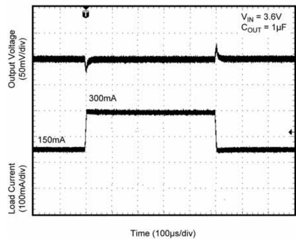
Load Transient
