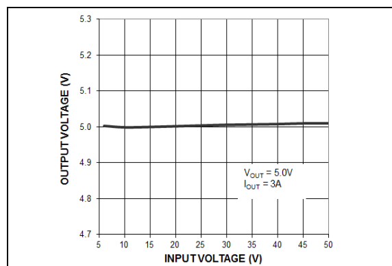
FIGURE 2-22: Output Voltage vs. Input Voltage (MIC28511-2).
