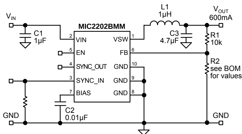
Figure 9. MIC2202BMM Schematic
