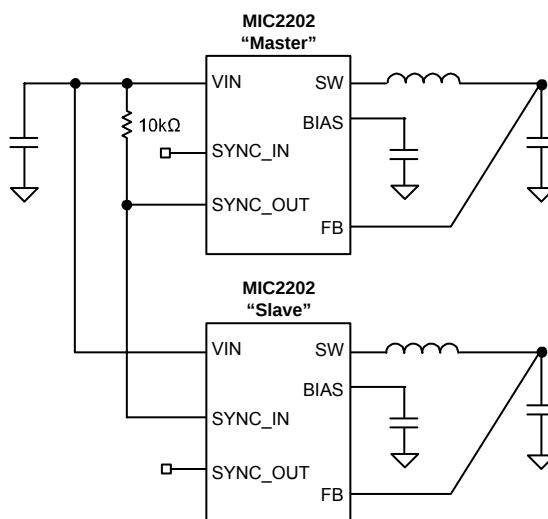
Figure 1. Master-Slave Operation
