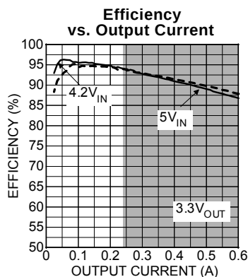
Figure 2. Efficiency Curve
