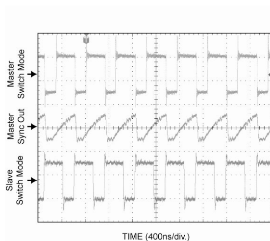
Figure 5. Master-Slave Synchronization Waveforms
