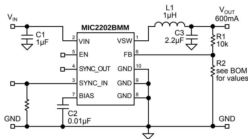
Figure 7. MIC2202BMM Schematic
