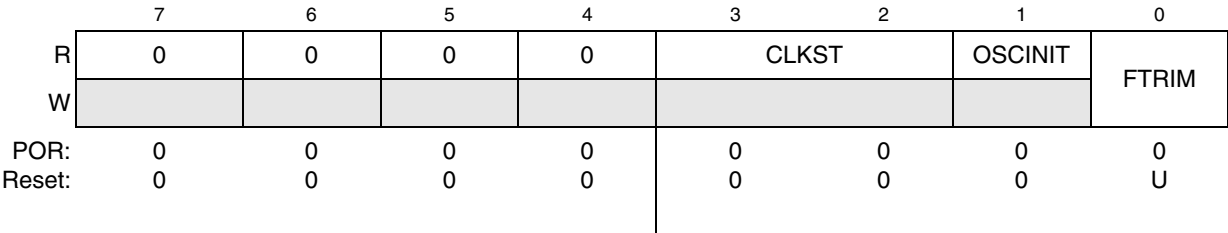
Figure 10-6. ICS Status and Control Register (ICSSC)
