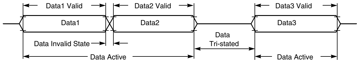
Figure 4. Signal states
