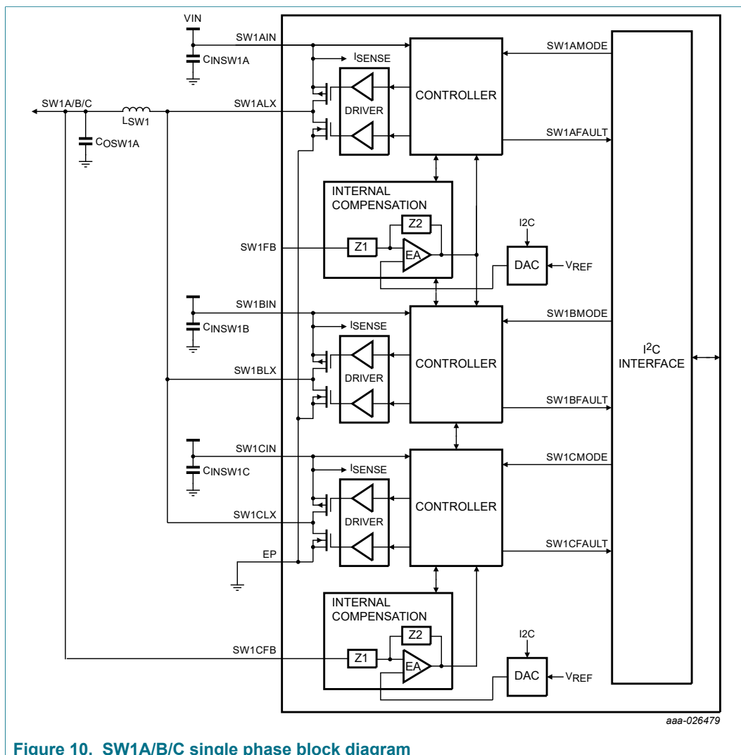
Figure 10. SW1A/B/C single phase block diagram
