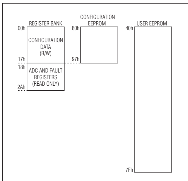
Figure 5. Memory Map
