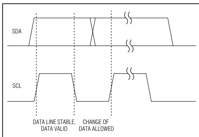
Figure 7. Bit Transfer
