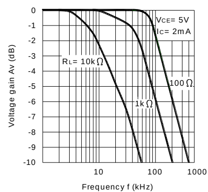
Fig.12 Frequency Response
