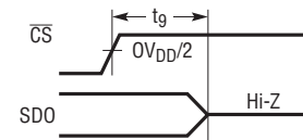
Figure 2. SDO Into Hi-Z after \overline{CS} ↑
