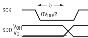
Figure 3. SDO Data Valid Hold after SCK↓
