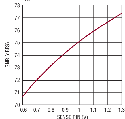
LTC2192: SNR vs SENSE, f_{IN} = 5\text{MHz} , -1dBFS
