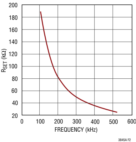
Figure 2. Timing Resistor (R SET ) Value
