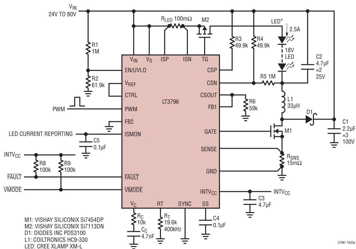
Buck Mode LED Driver with Open LED Flag and LED Current Reporting
