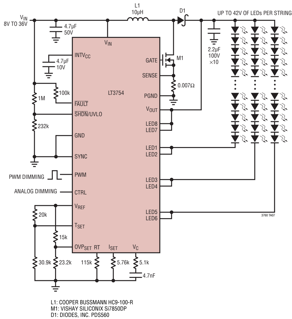
25W LED Driver, 400kHz Boost, 3 Strings, 200mA Per String
