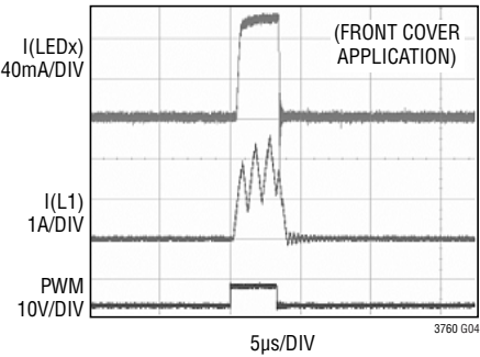
LED Current Waveforms 3000:1 PWM Dimming (100Hz)
