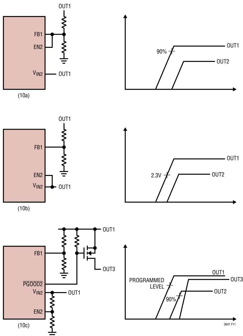
Figure 10. The EN2 and PG00D2 Pins Allow Serial Sequencing Options
