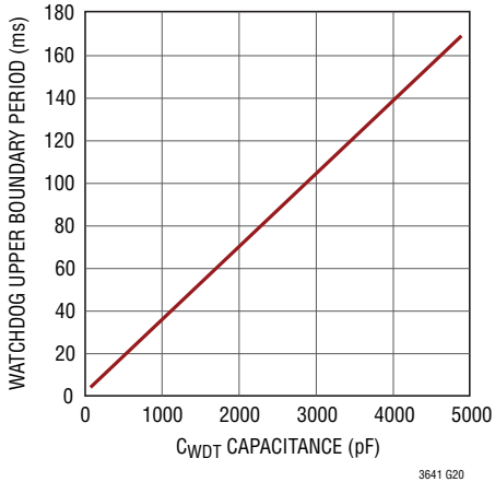
Watchdog Upper Boundary Period vs C_{WDT}
