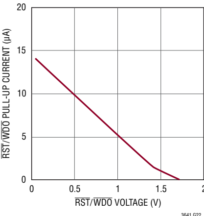
\overline{\text{RST}}/\overline{\text{WDO}} Pull-Up Current
