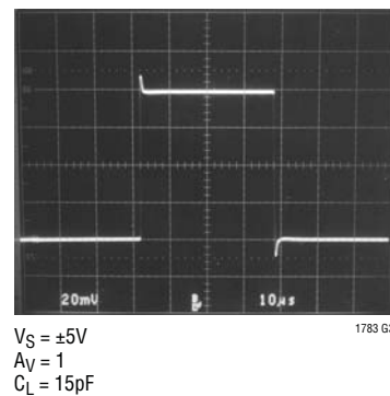
Small-Signal Response
