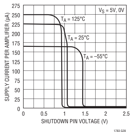
Supply Current vs SHDN Pin Voltage
