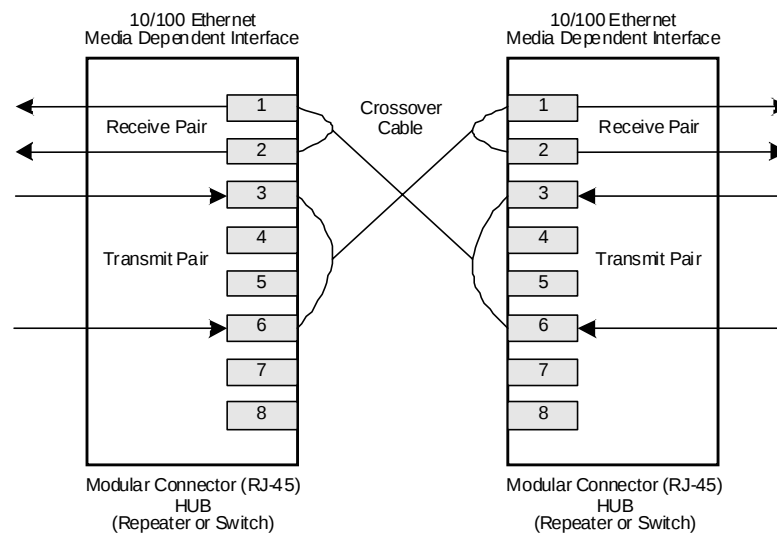
Figure 5. Typical Crossover Cable Connection
