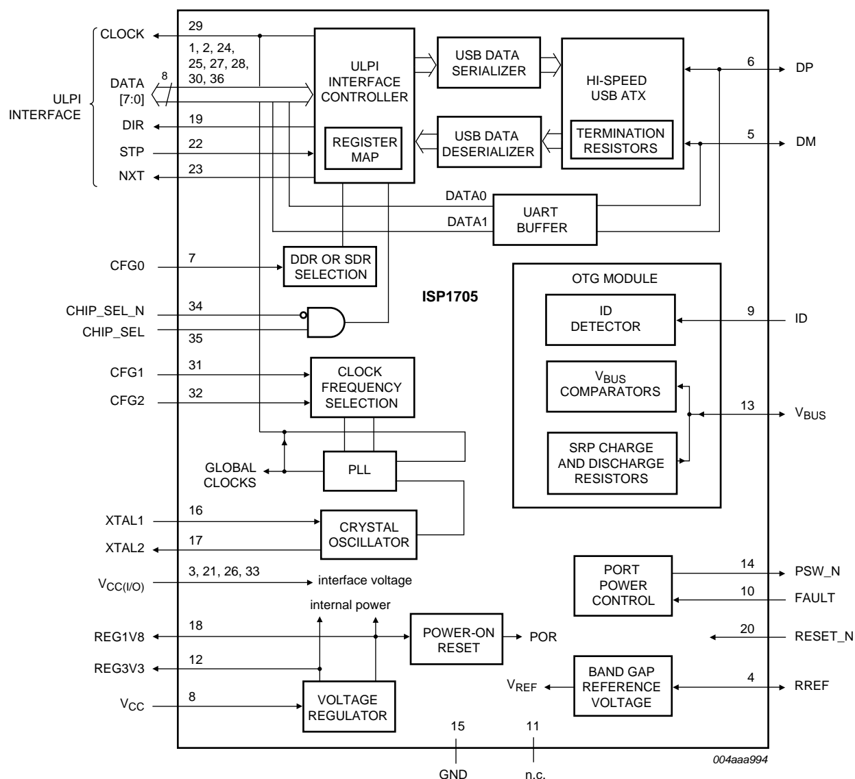
Fig 1. Block diagram
