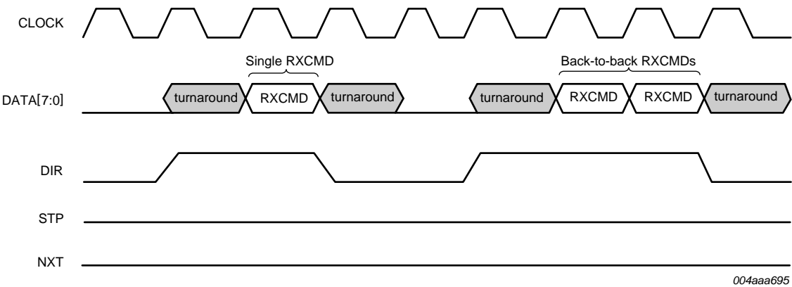
Fig 12. Single and back-to-back RXCMDs from the ISP1705 to the link
