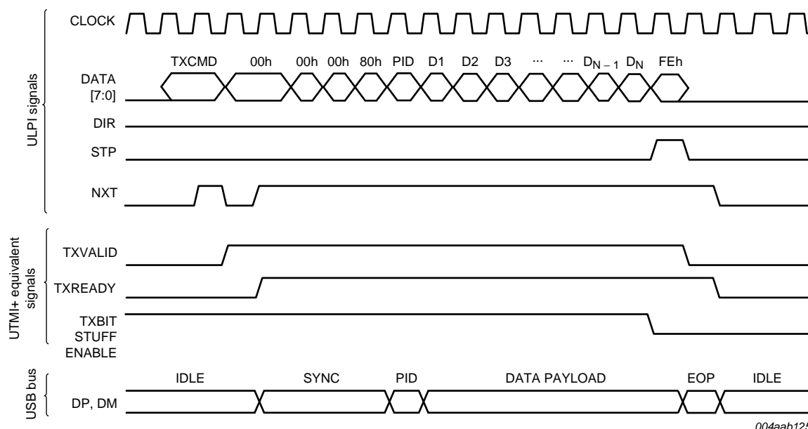
Fig 23. Transmitting USB packets without automatic SYNC and EOP generation
