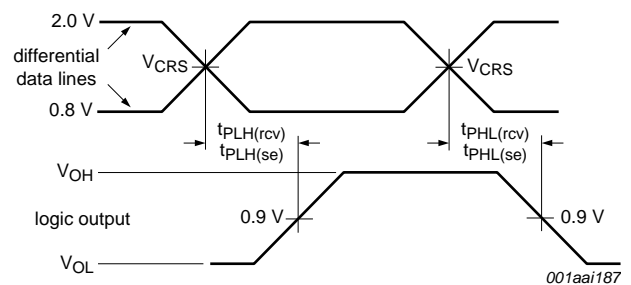
Fig 29. Timing of DP and DM to RX_RCV, RX_DP and RX_DM
