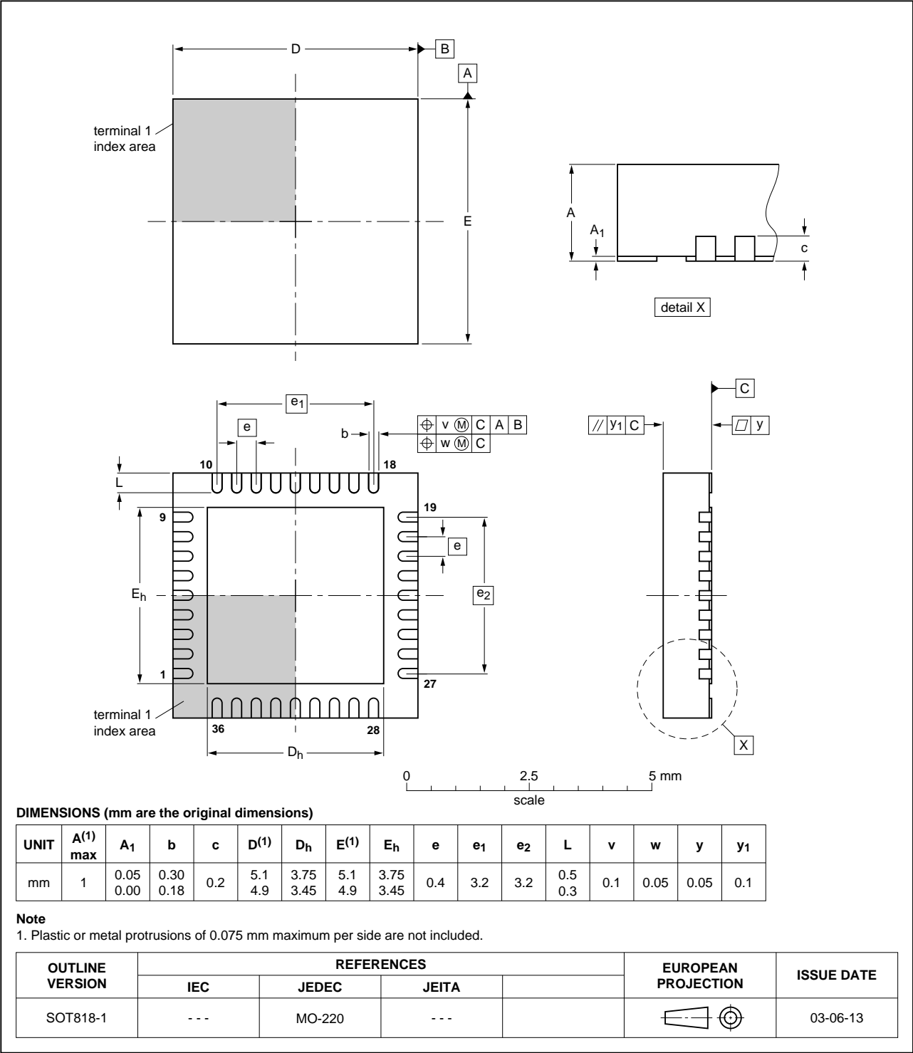
Fig 34. Package outline SOT818-1 (HVQFN36)
