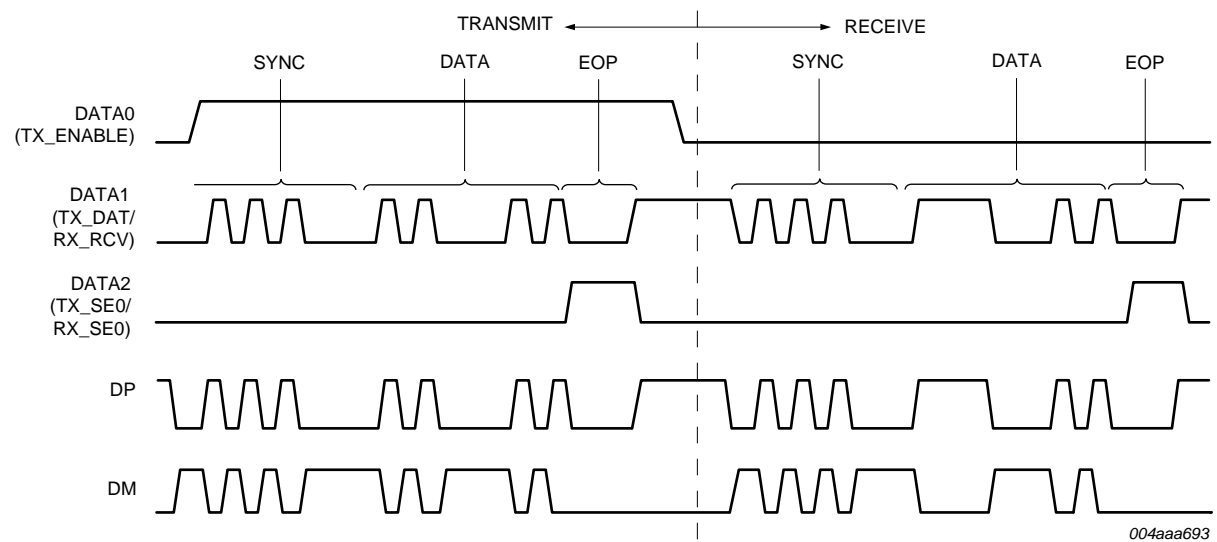
Fig 25. Example of transmit followed by receive in 3-pin serial mode
