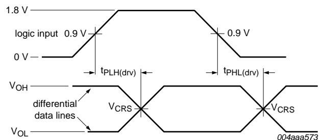
Fig 27. Timing of TX_DAT and TX_SE0 to DP and DM
