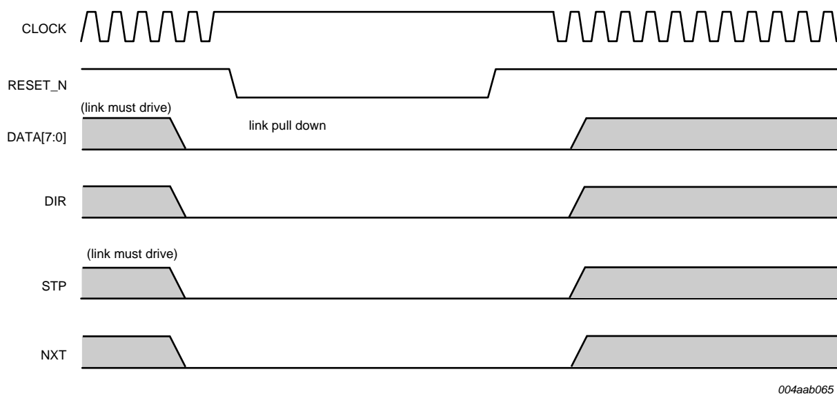
Fig 7. Interface behavior with respect to RESET_N during normal mode
