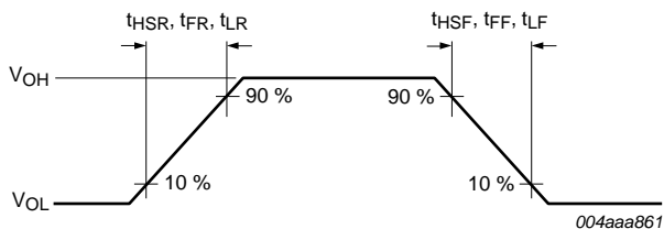
Fig 26. Rise time and fall time
