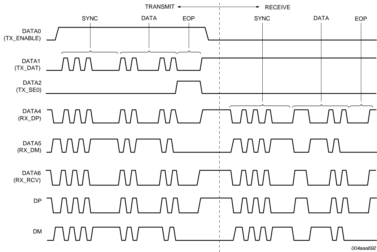
Fig 24. Example of transmit followed by receive in 6-pin serial mode
