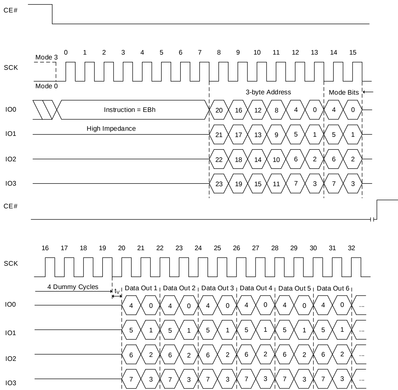
Figure 8.7.1 Fast Read Quad I/O Sequence (with command decode cycles)
