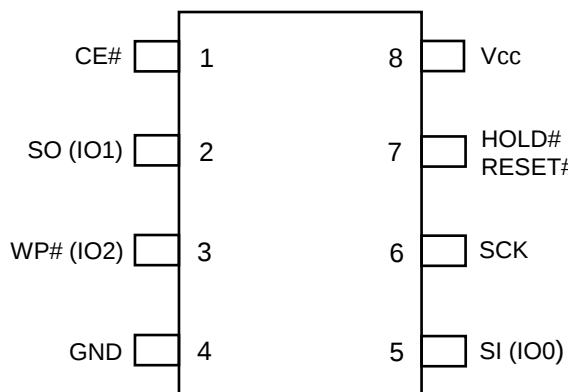
8-pin SOIC 208mil (Package: B) 8-pin SOIC 150mil (Package: N)
