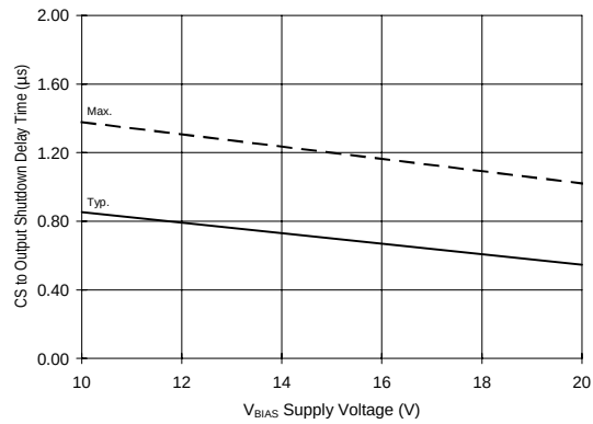
Figure 12B. CS to Output Shutdown Delay Time vs. Voltage
