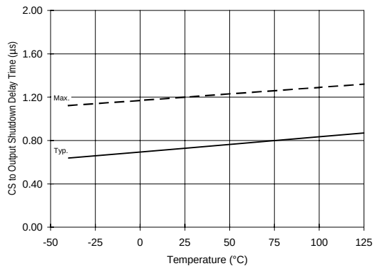
Figure 12A. CS to Output Shutdown Delay Time vs. Temperature
